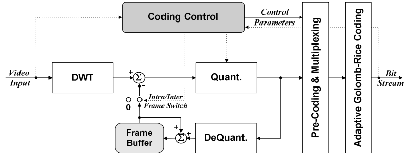
Figure 1: Block diagram of our proposed video coding scheme.
