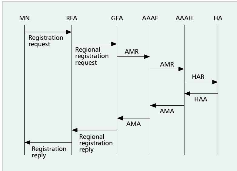
■ Figure 2. Mobile IP registration.
