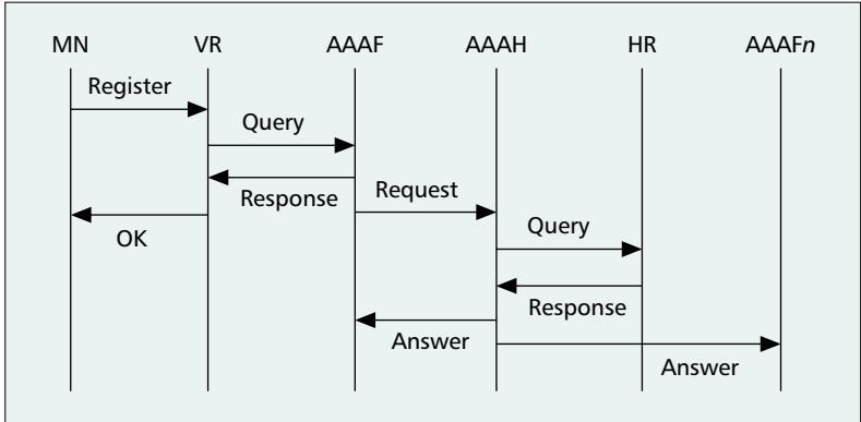
■ Figure 7. SIP interdomain handoff with Shadow Registration.
