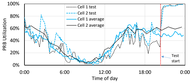
Figure 1: Large downloads start at 20:45 UTC in two cells and last for 4 hours, consuming nearly all available resources.
