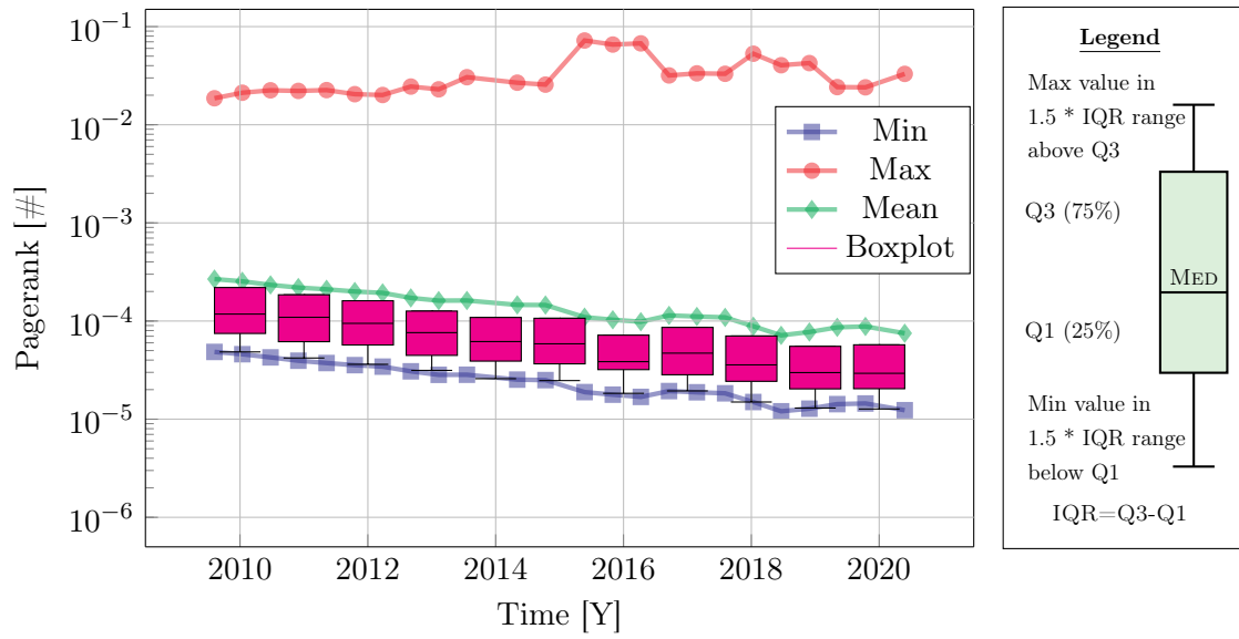
Figure 4.16: P2P relationships
