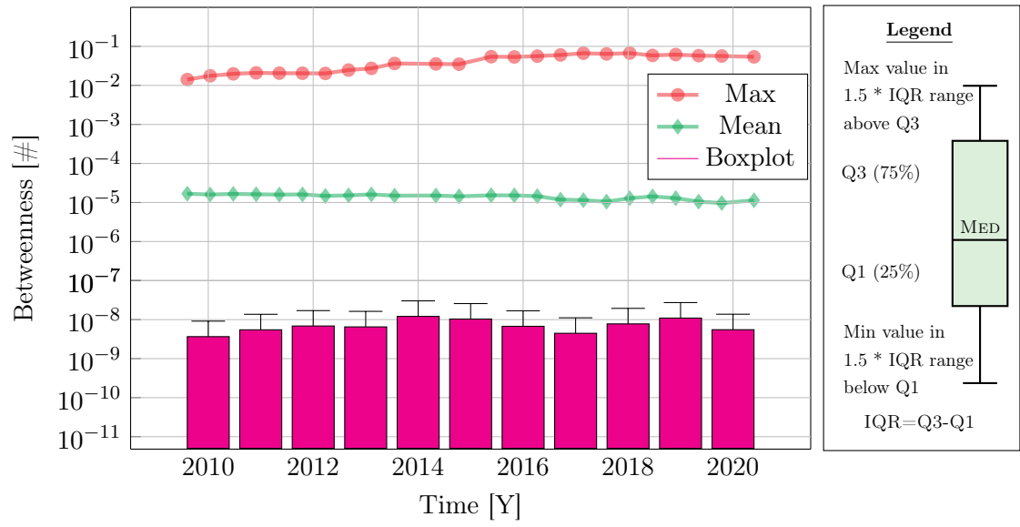
Figure 4.29: All relationships (Only ISPs)
