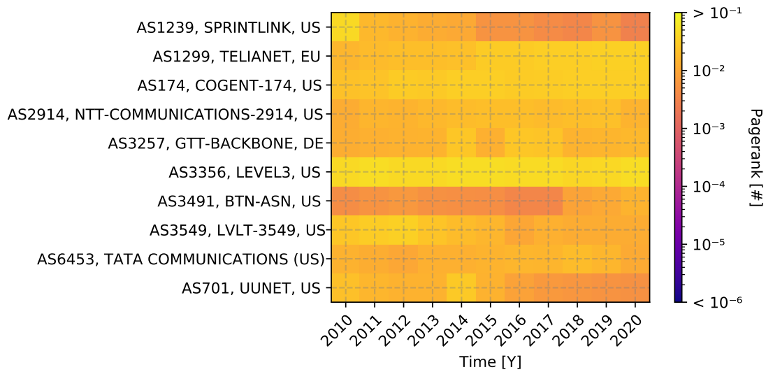
Figure 4.15: Cumulative top five ASes by pagerank values of C2P relationships
