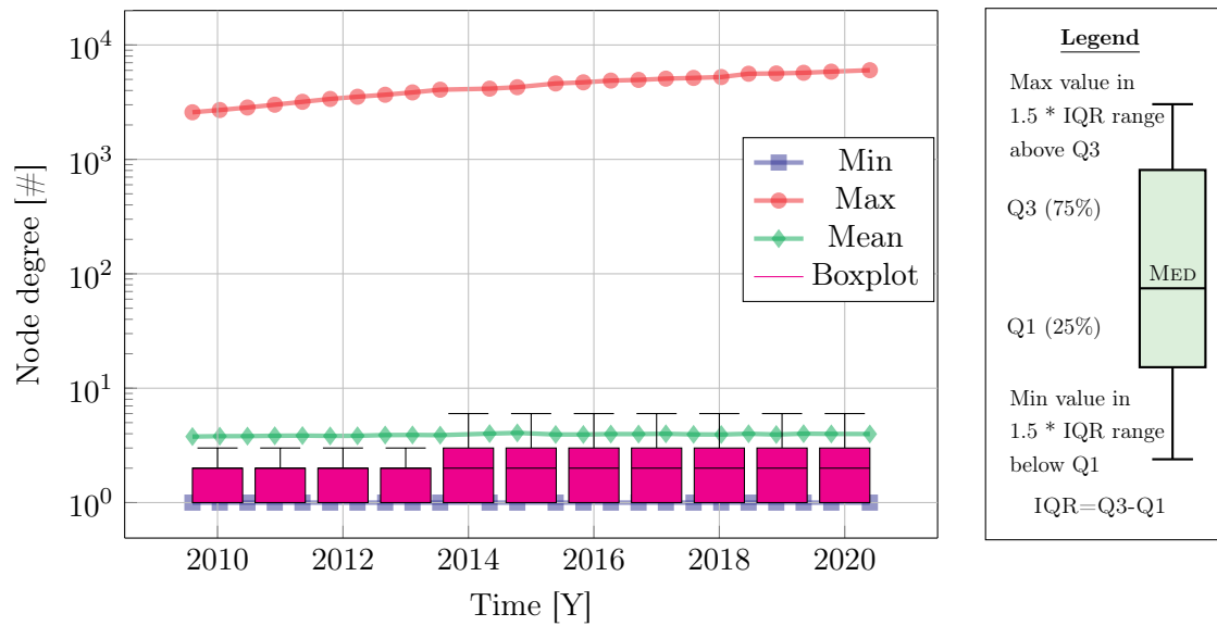
Figure 4.8: Total average node degree of C2P relationships
