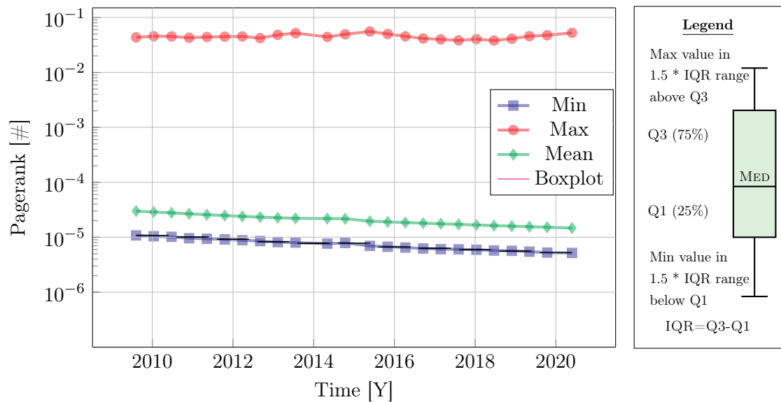
Figure 4.13: C2P relationships
