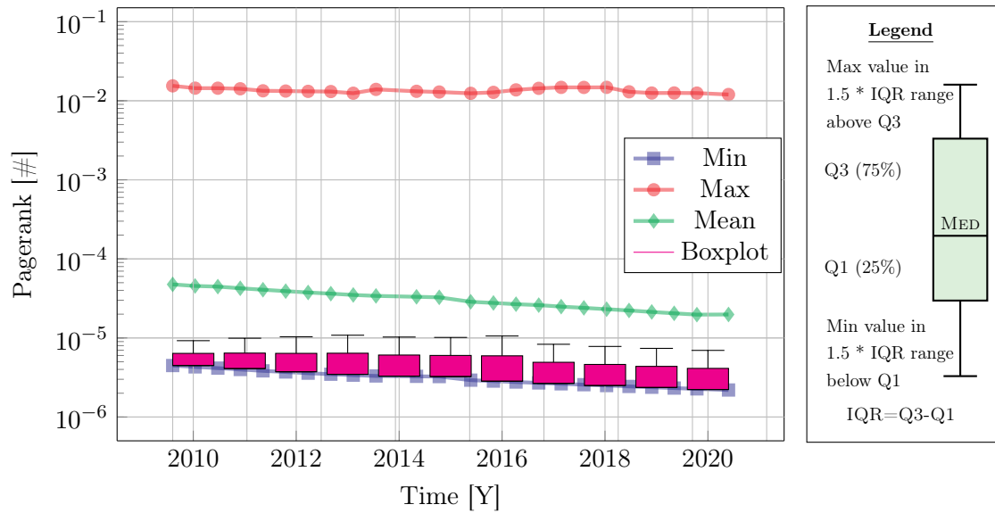
Figure 4.20: All relationships (Only ISPs)
