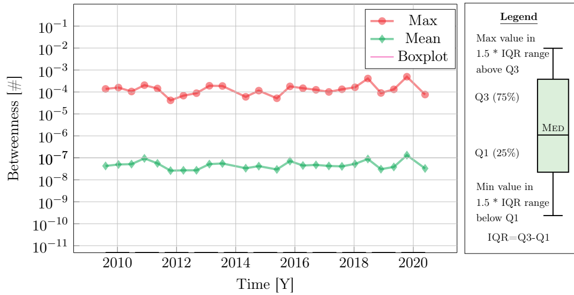
Figure 4.22: C2P relationships
